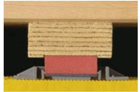
J-Lock component in unloaded position.
