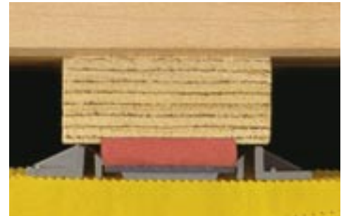
J-Lock component with maximum load (note that the J-Locks will never be provoked to this deformation extent by the athlete).
